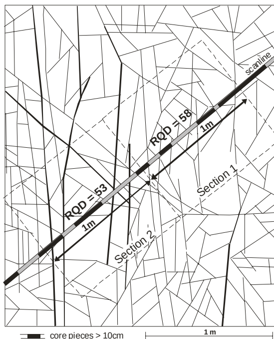
Figure 10. By applying a scanline in Figure 2, the RQD-values can be found. "Core pieces" > 10cm are shown in black. However, this measurement does not show the large variation in block sizes as is seen in Figure 5.
