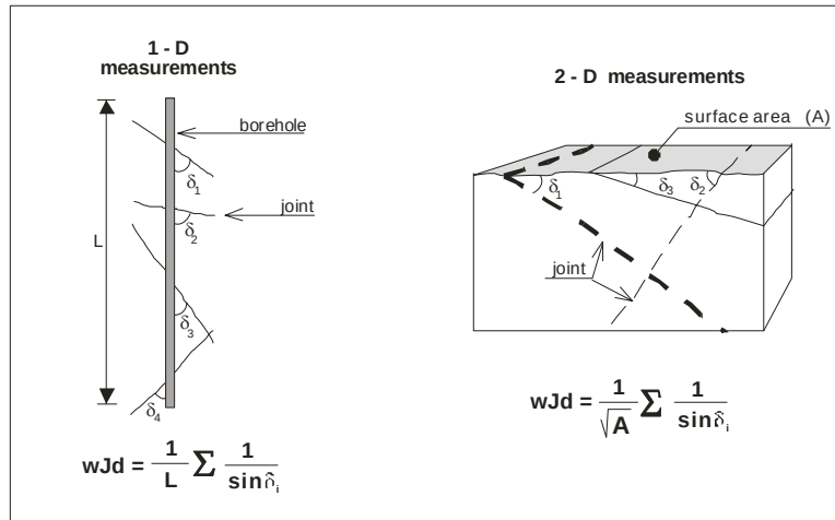
Figure 8. The definitions of wJd measurement for borehole and surface registrations. (Palmstrom, 1995).
