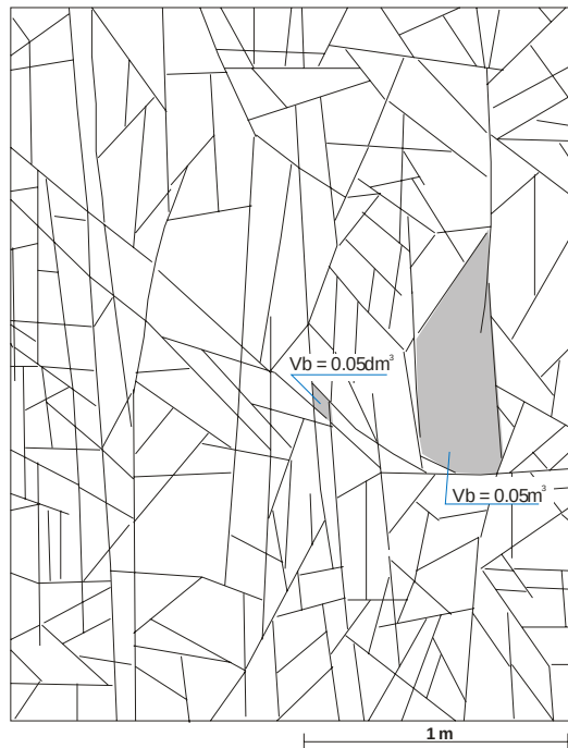
Figure 5. The block volumes in Figure 2 vary between approx. 5 \times 10^{-5}\text{m}^3 and 5 \times 10^{-2}\text{m}^3 . Average block size \approx 0.025\text{m}^3 .
